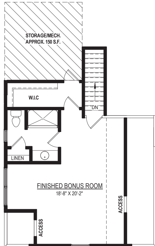
OPT. FINISHED SECOND FLOOR PLAN W/ OPT. DOUBLE DORMER & OPT. FULL BATH
