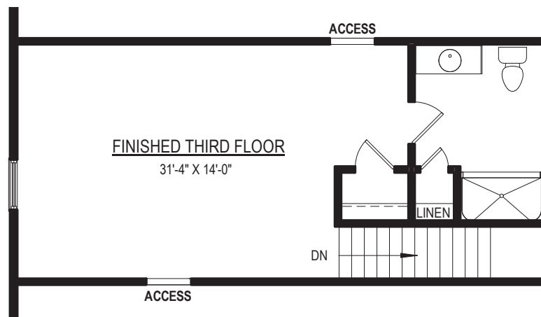
OPT. FINISHED THIRD FLOOR W/ FULL BATH
