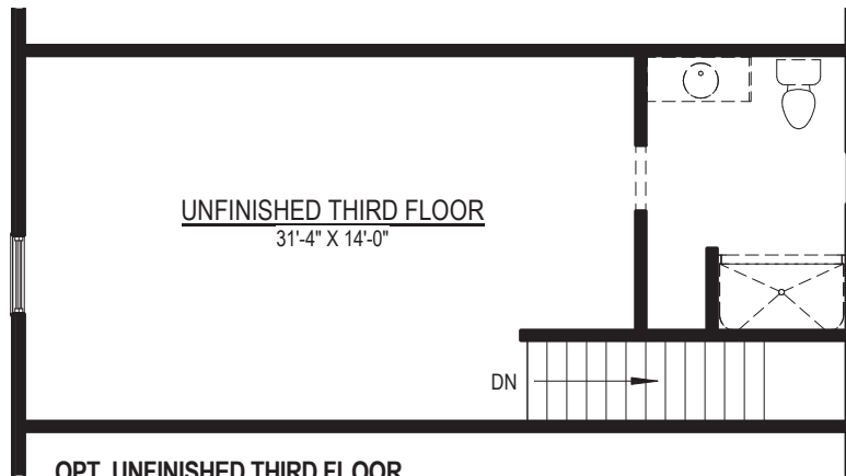
OPT. UNFINISHED THIRD FLOOR W/ OPT. FULL BATH ROUGH-IN
